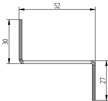
Jamb flashing profile (sides)
