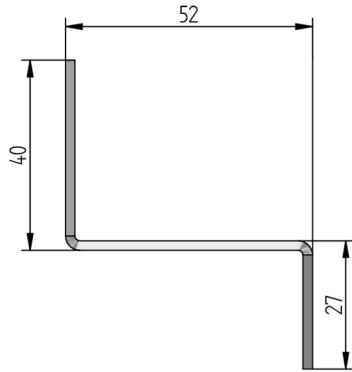
Head flashing profile (top)
