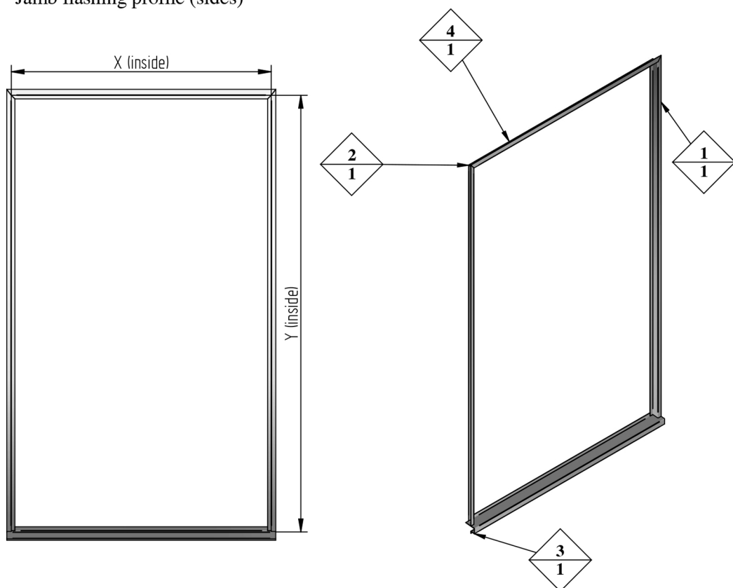
Jamb flashing profile (sides)
