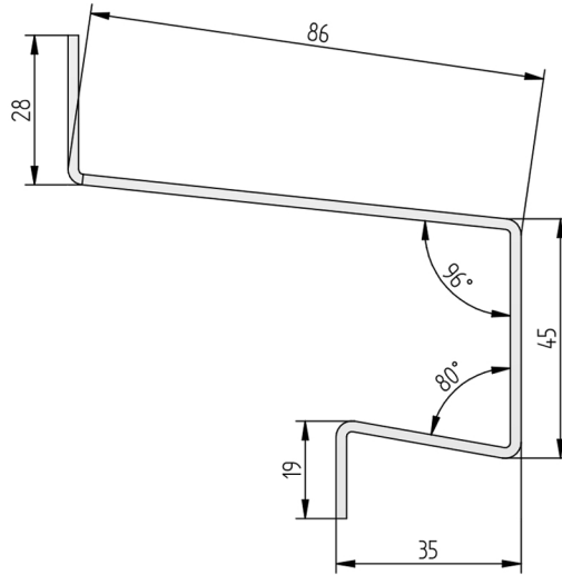
Sill flashing profile (bottom)
