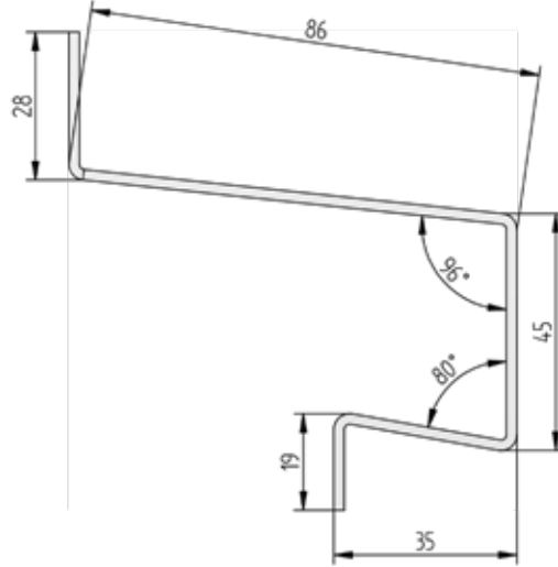
Sill flashing profile (bottom)
